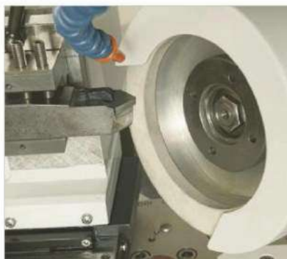
PCD 刀片磨削 PCD inserts grinding
