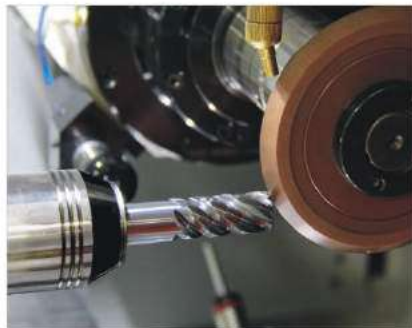
容屑槽磨削 Gash grinding
